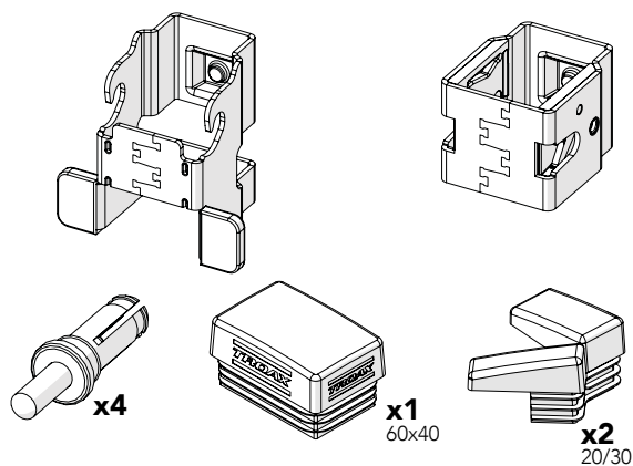
Kit Rapid Fix bracket 36701060
